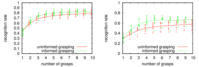
Fig. 6: Comparison of the uninformed and informed grasping strategy depending on the number of grasps. Left: household + industrial objects (full data set) Right: industrial objects only
